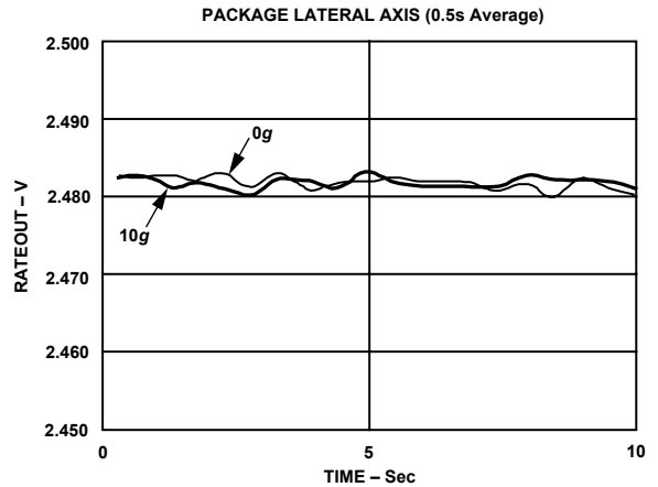
Figure 12. 10 g Random Vibration in Package-Lateral Axis Orientation
