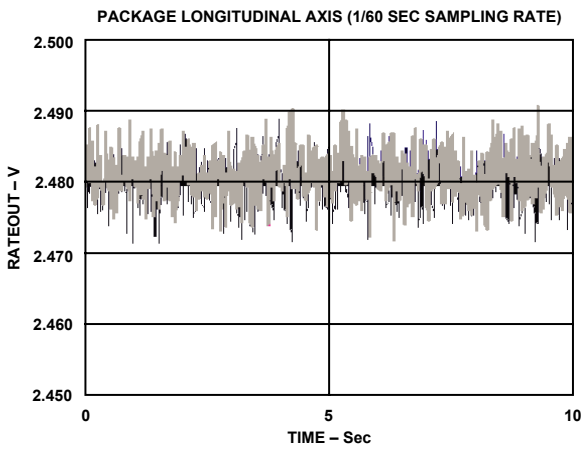
Figure 10. 10 g Random Vibration in Package-Longitudinal Axis Orientation
