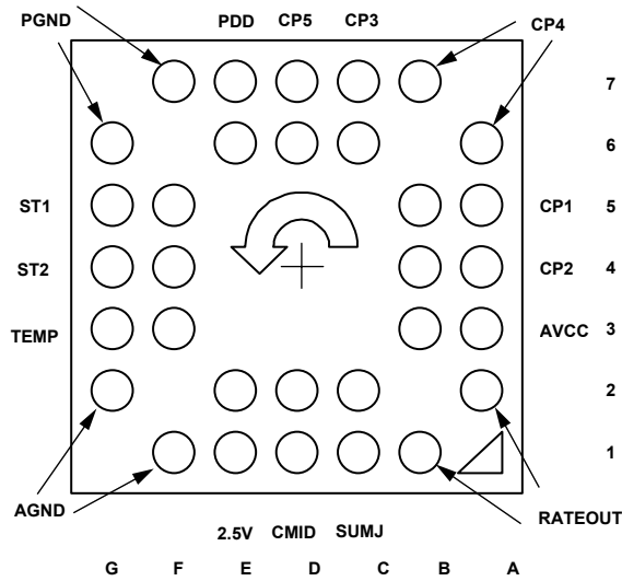
Figure 5. BGA-32 (Bottom View)
